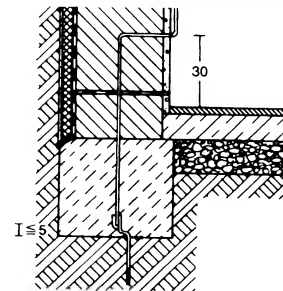
⑫ Earthing electrode in a foundation of unreinforced concrete
